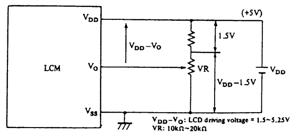
Fig. 4 Power supply
