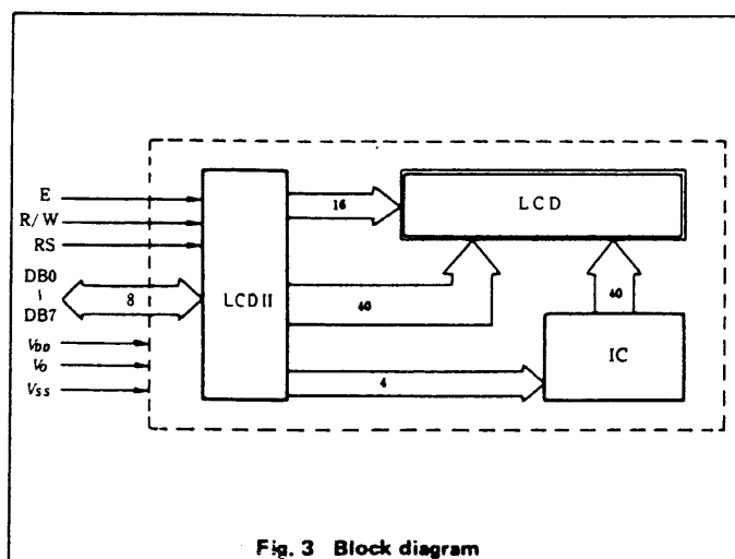
Fig. 3 Block diagram
